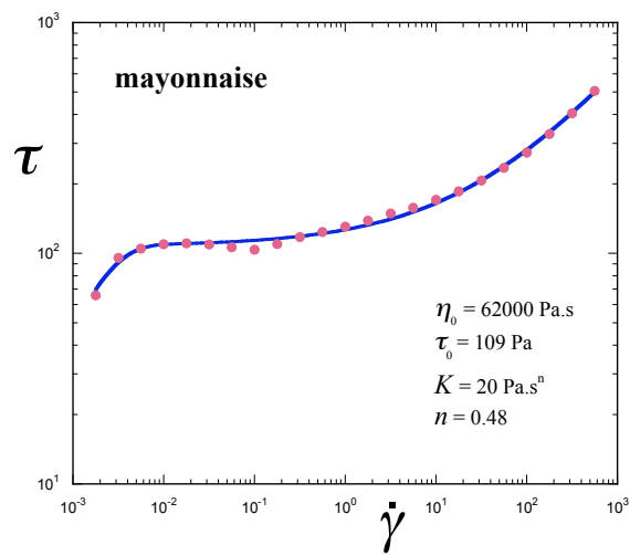
Figure 9: Flow curve of mayonnaise.
