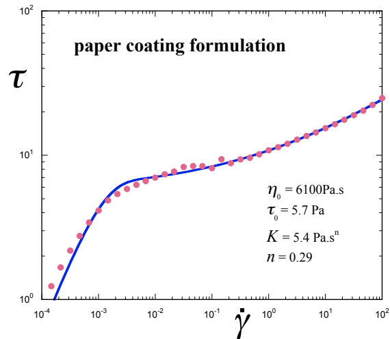
Figure 10: Flow curve of a paper coating formulation.
